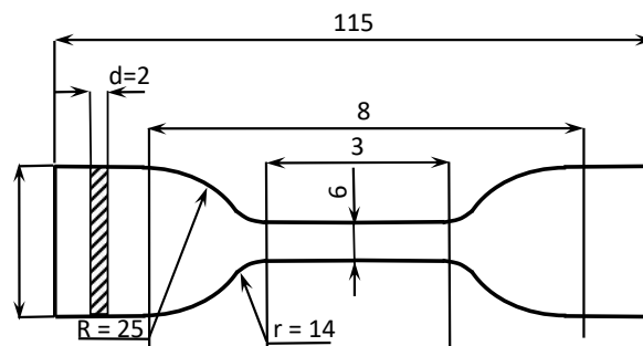
Fig. 5. Test sample in the form of a bilateral blade
